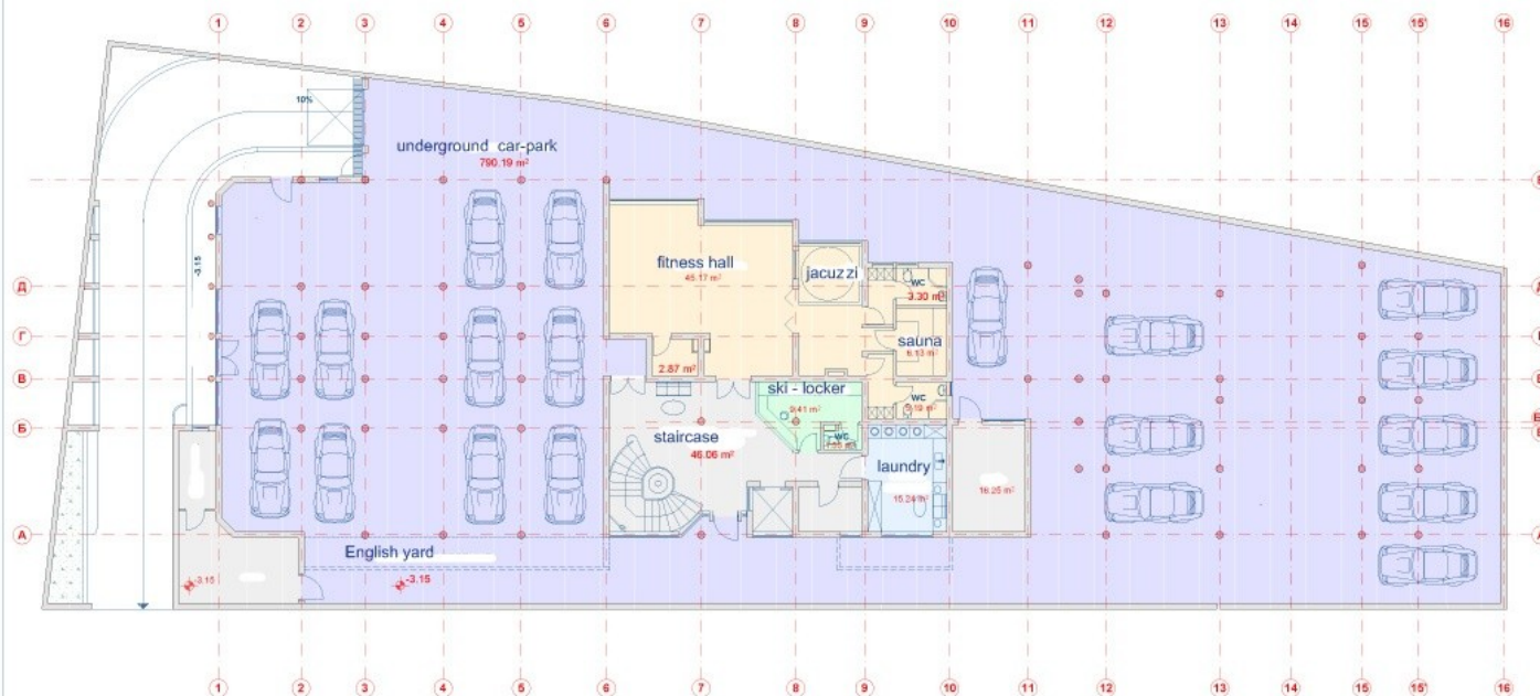
UNDER-GROUND FLOOR PLAN
